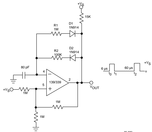
Figure 15. Pulse Generator
